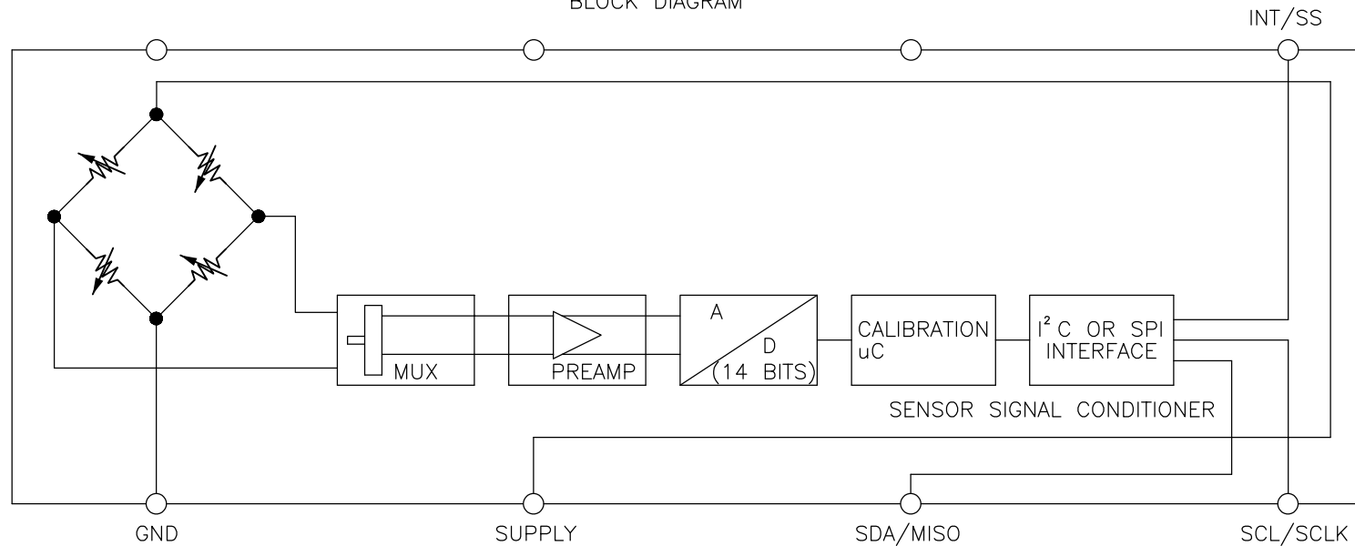
BLOCK DIAGRAM
