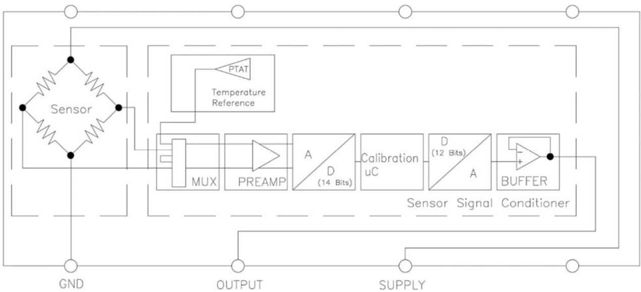
SA18 Analog output
