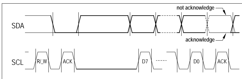
Each byte is followed by an acknowledge or a not acknowledge, generated by the receiver
