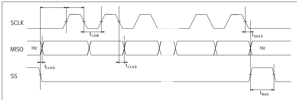
SPI Timing Diagram
