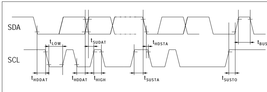
I2C Timing Diagram
