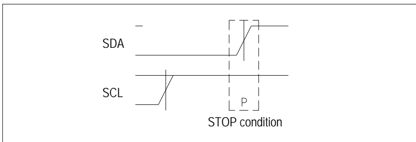
A LOW to HIGH transition on the SDA line while SCL is HIGH
